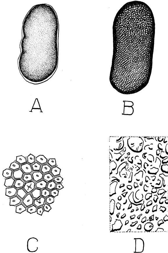
FIG. 1. A .—A young statoblast of Fredericella sultana . The unattached surface is quite smooth. Dimensions 0.4176 mm. long, 0.1914 mm. wide. B .—An older statoblast of F. sultana . C .—An enlarged drawing of the surface of B . D .—A portion of the roughened surface of an old statoblast of F. sultana . The magnification is the same as in C . All figures were made with the aid of a camera lucida.
